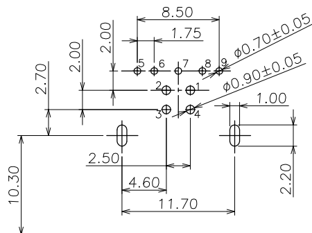
PCB LAYOUT(TOP VIEW T=1.60)
