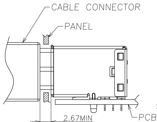
RECESSED MOUNTING CONFIGURATION
