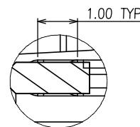
Detail "C" SCALE 4:1
