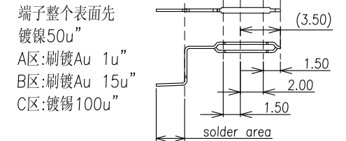
CONTACT PLATING DIAGRAM
