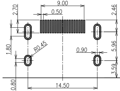
PCB LAYOUT(TOP VIEW T1.6)
