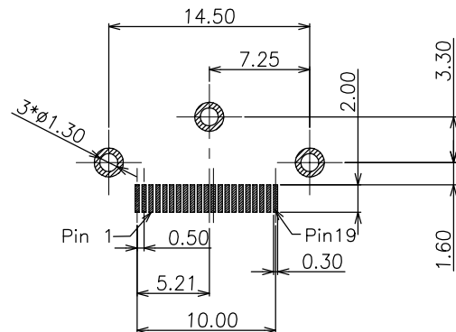
PCB LAYOUT(TOP VIEW T1.6)
