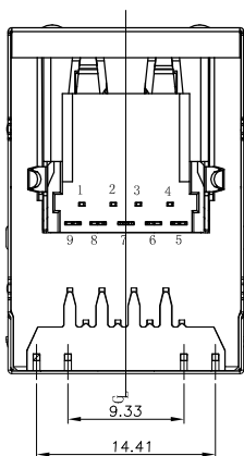
BOTTOM VIEW
