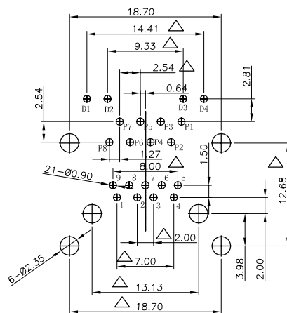
RECOMMENDED P.C.B LAYOUT TOP VIEW (COMPONENT SIDE)
