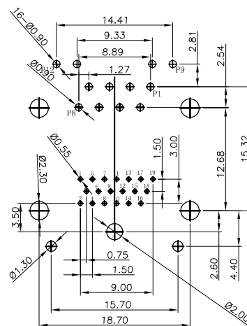
RECOMMENDED P.C.B LAYOUT TOP VIEW (COMPONENT SIDE)
