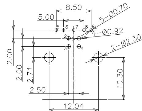
PCB LAYOUT(TOP VIEW T=1.20)
