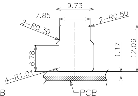
MOUNTING PANEL CUTOUT(INTERNAL SIDE)
