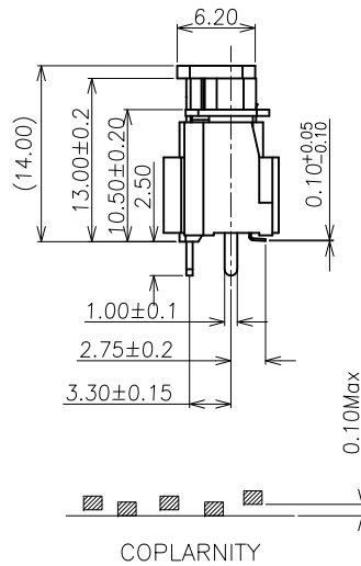
COPLANARITY
