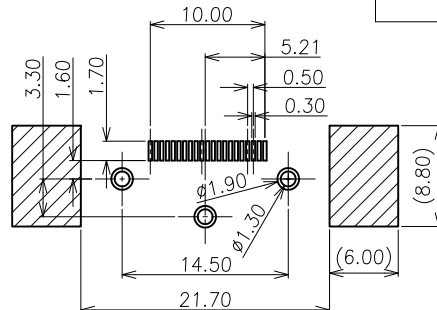
PCB LAYOUT(TOP VIEW) (T=1.60mm)
