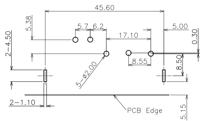
PCB LAYOUT TOP VIEW(T1.6)
