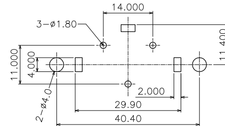
PCB CUT-OUT
