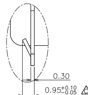
DETAIL A (4:1)
